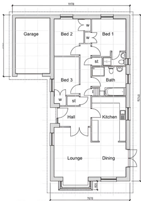
Floor Plan as Proposed
