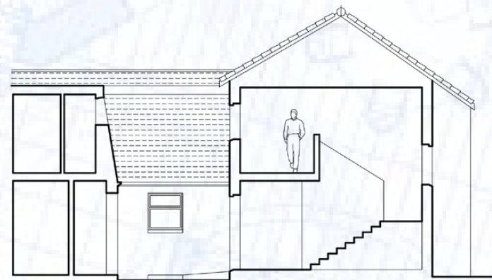
CROSS SECTION THROUGH MAIN STAIR AS EXISTING
