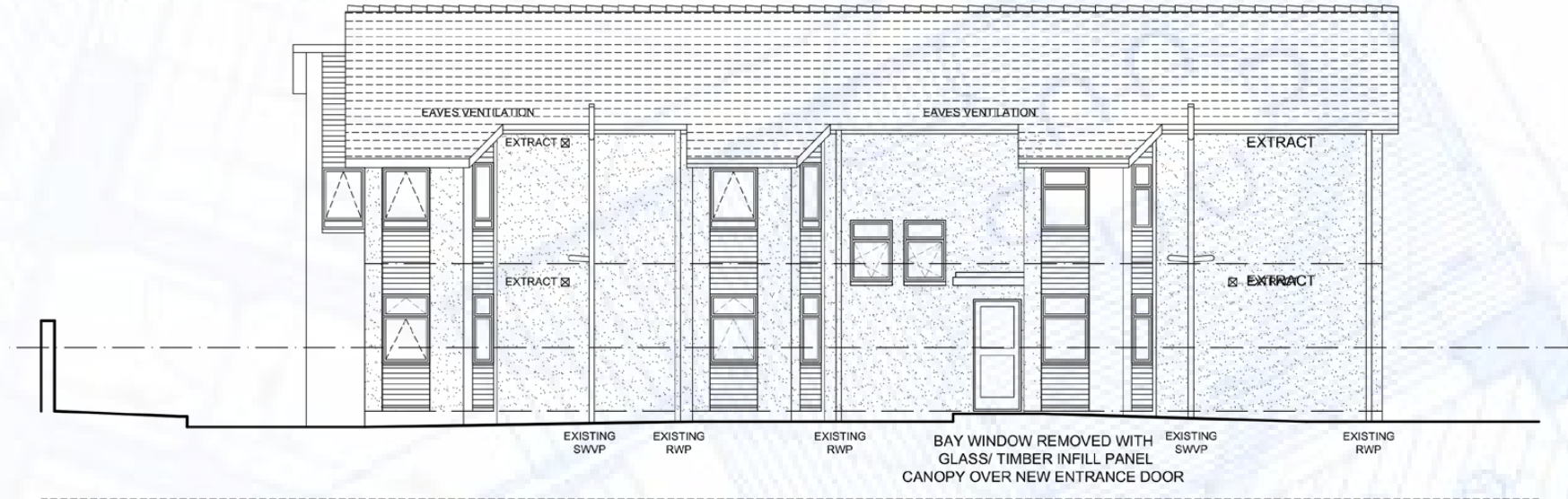
NORTH ELEVATION AS PROPOSED
