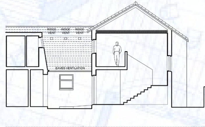
CROSS SECTION THROUGH MAIN STAIR AS PROPOSED
