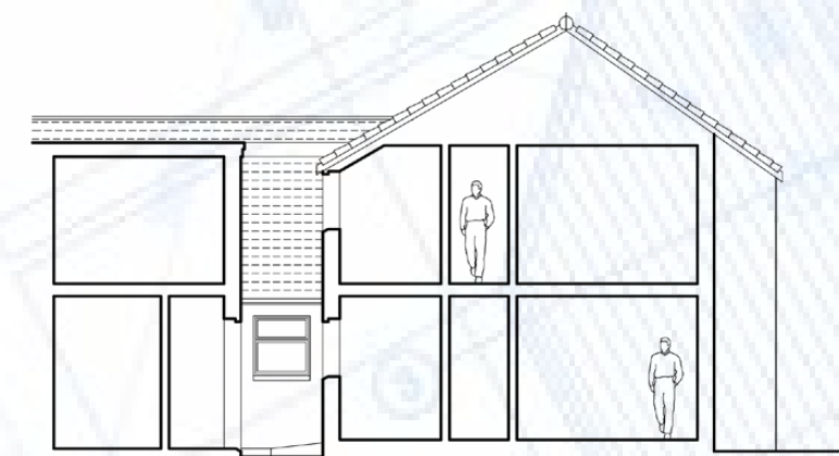
CROSS SECTION THROUGH MAIN BUILDING AS EXISTING
