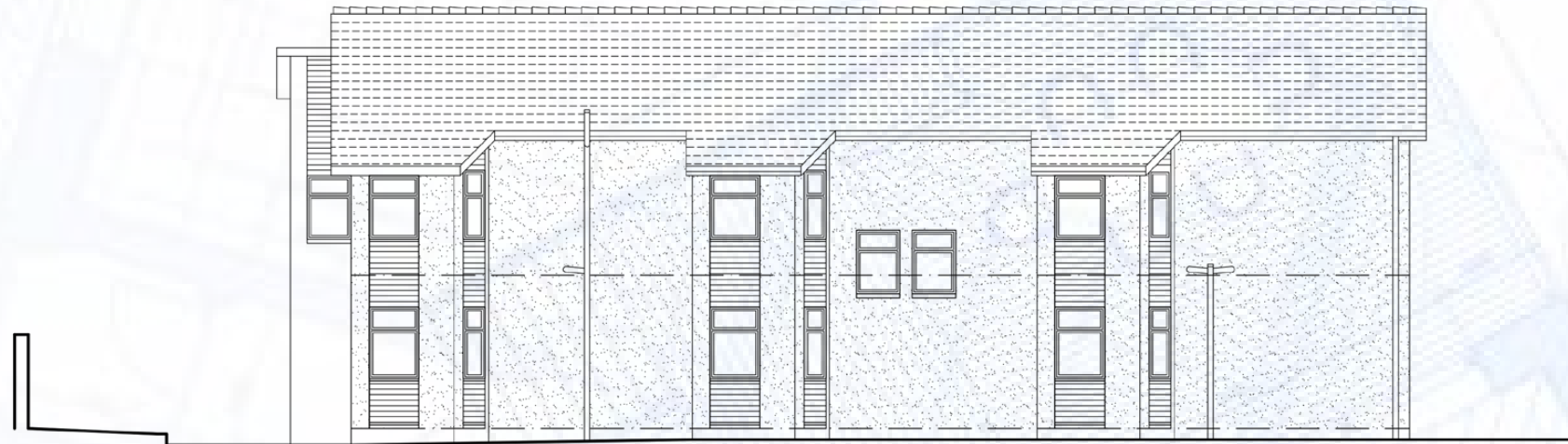
NORTH ELEVATION AS EXISTING
