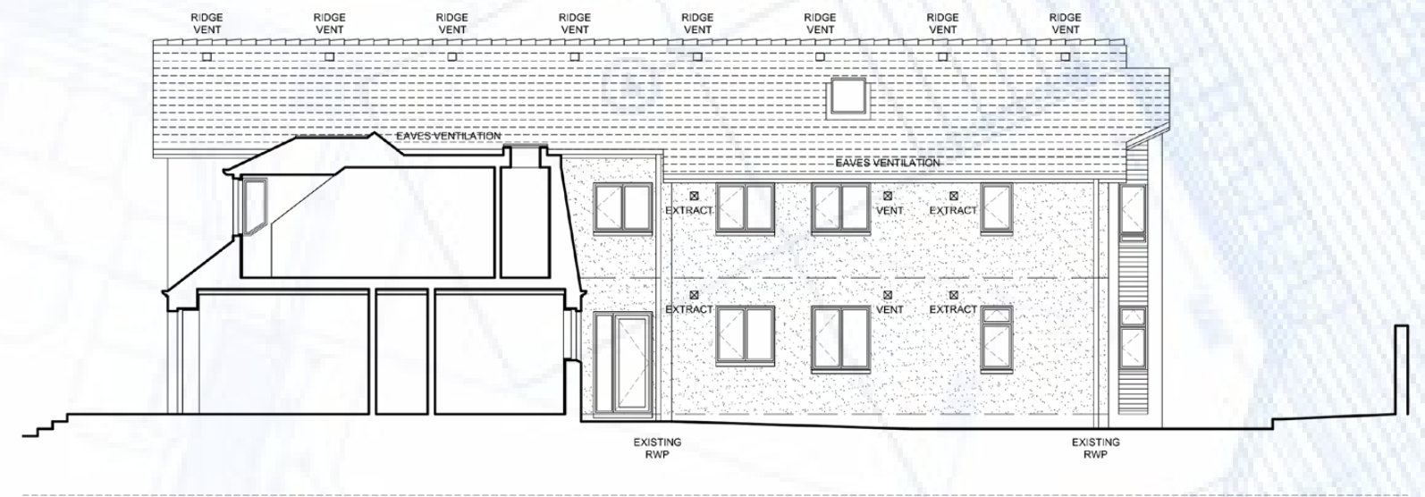
CROSS SECTION THROUGH COTTAGE AS PROPOSED
