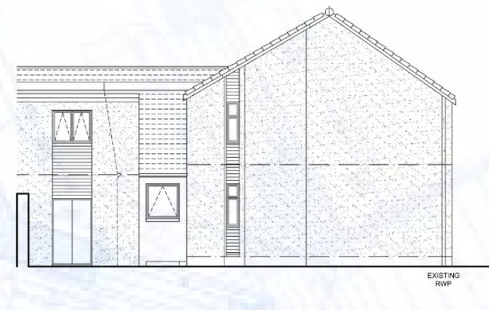
REAR ELEVATION AS PROPOSED
