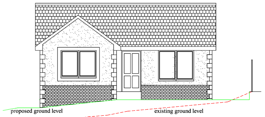
FRONT ELEVATION
