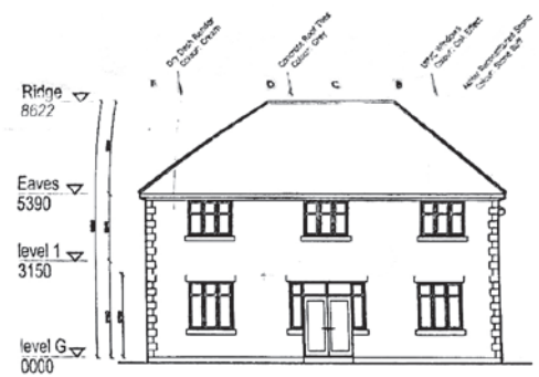
Rear Elevation Scale 1:100
