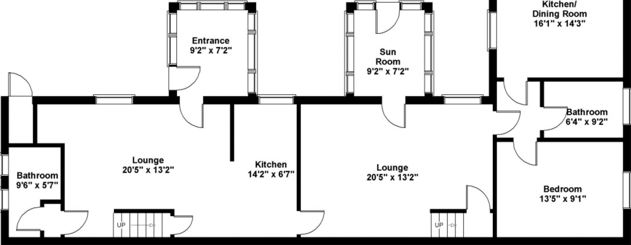
GROUND FLOOR
