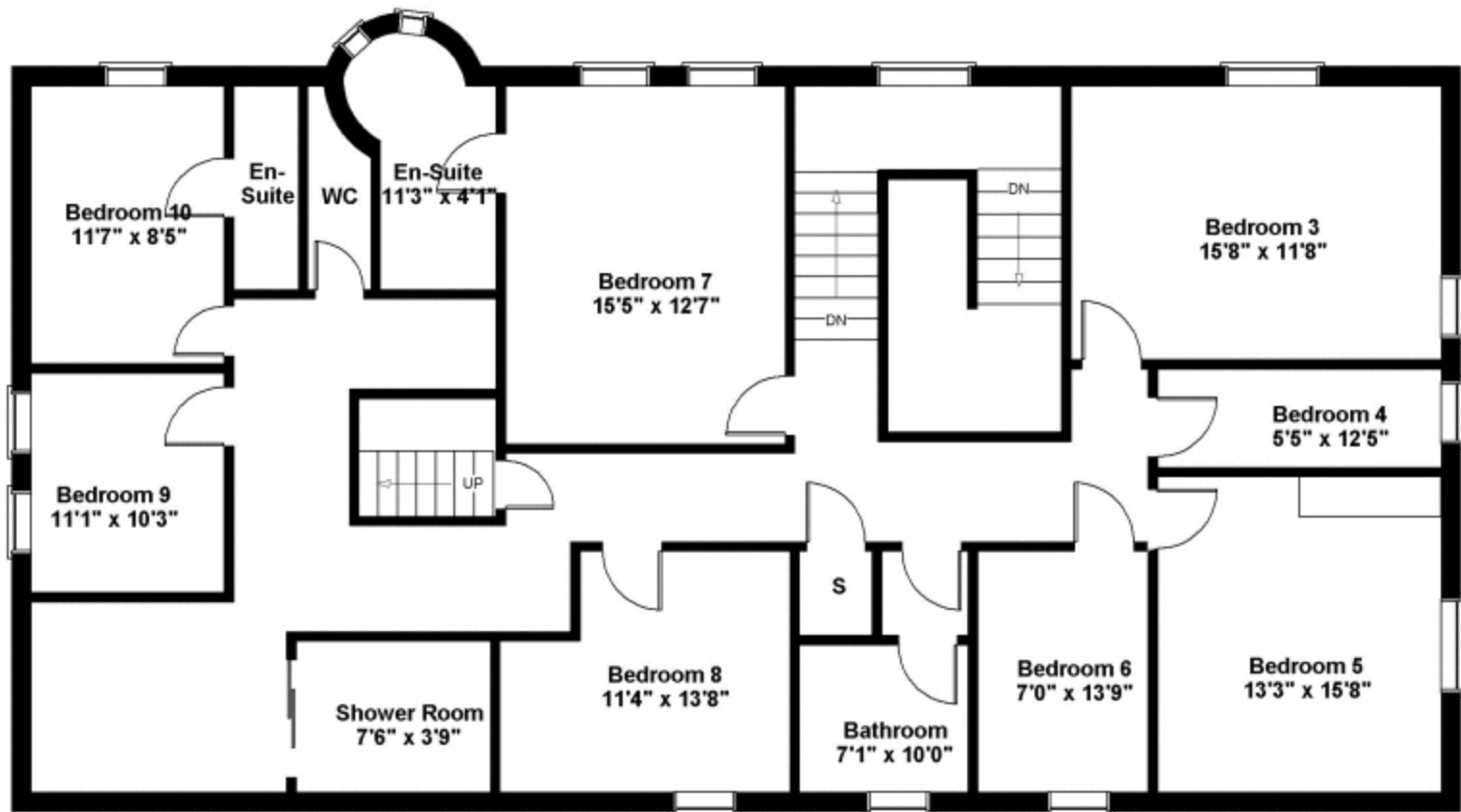
FIRST FLOOR
