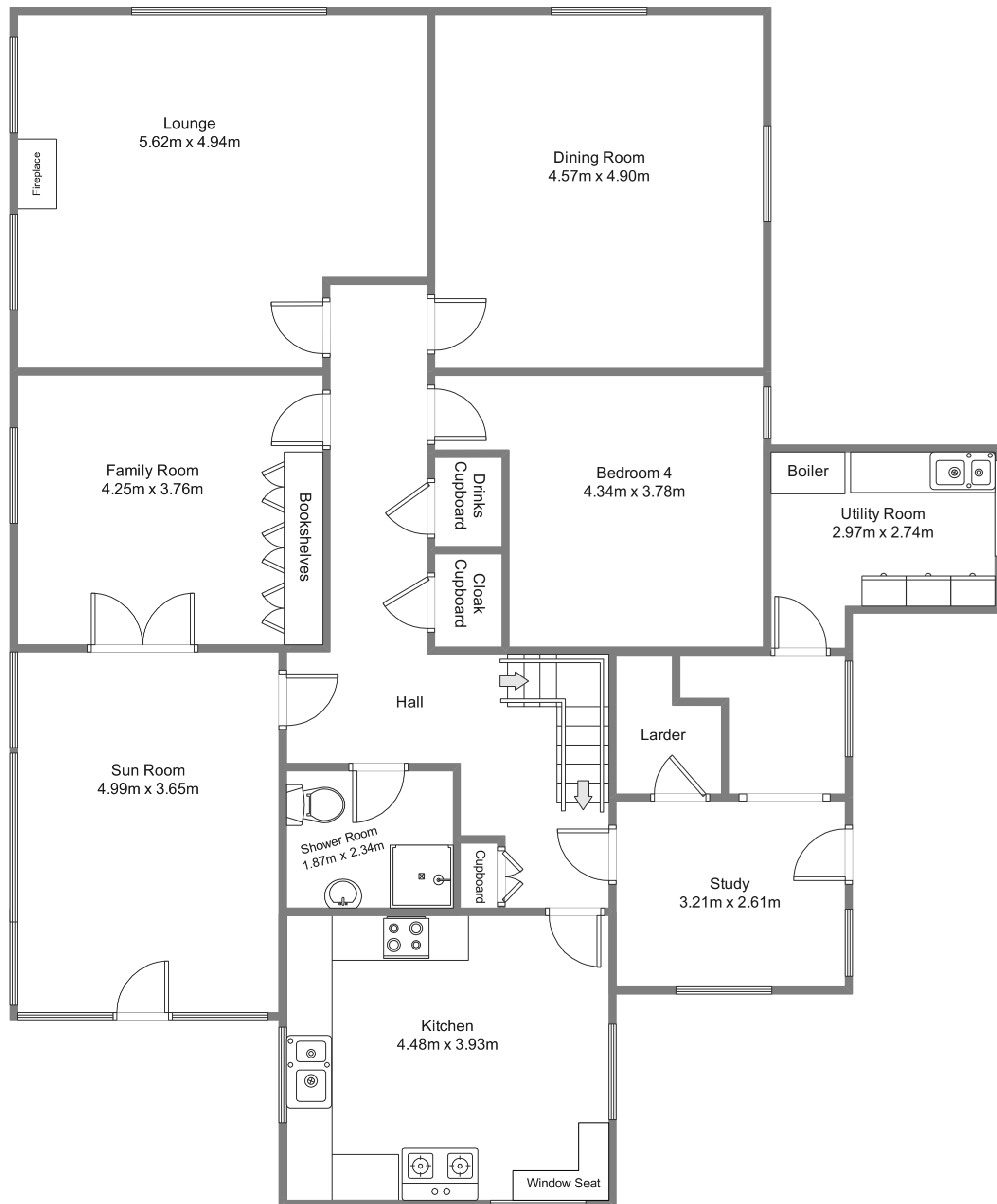
Ground Floor
