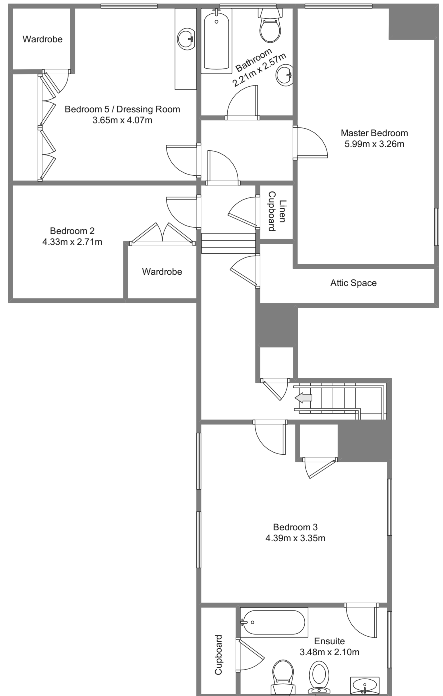
First Floor
