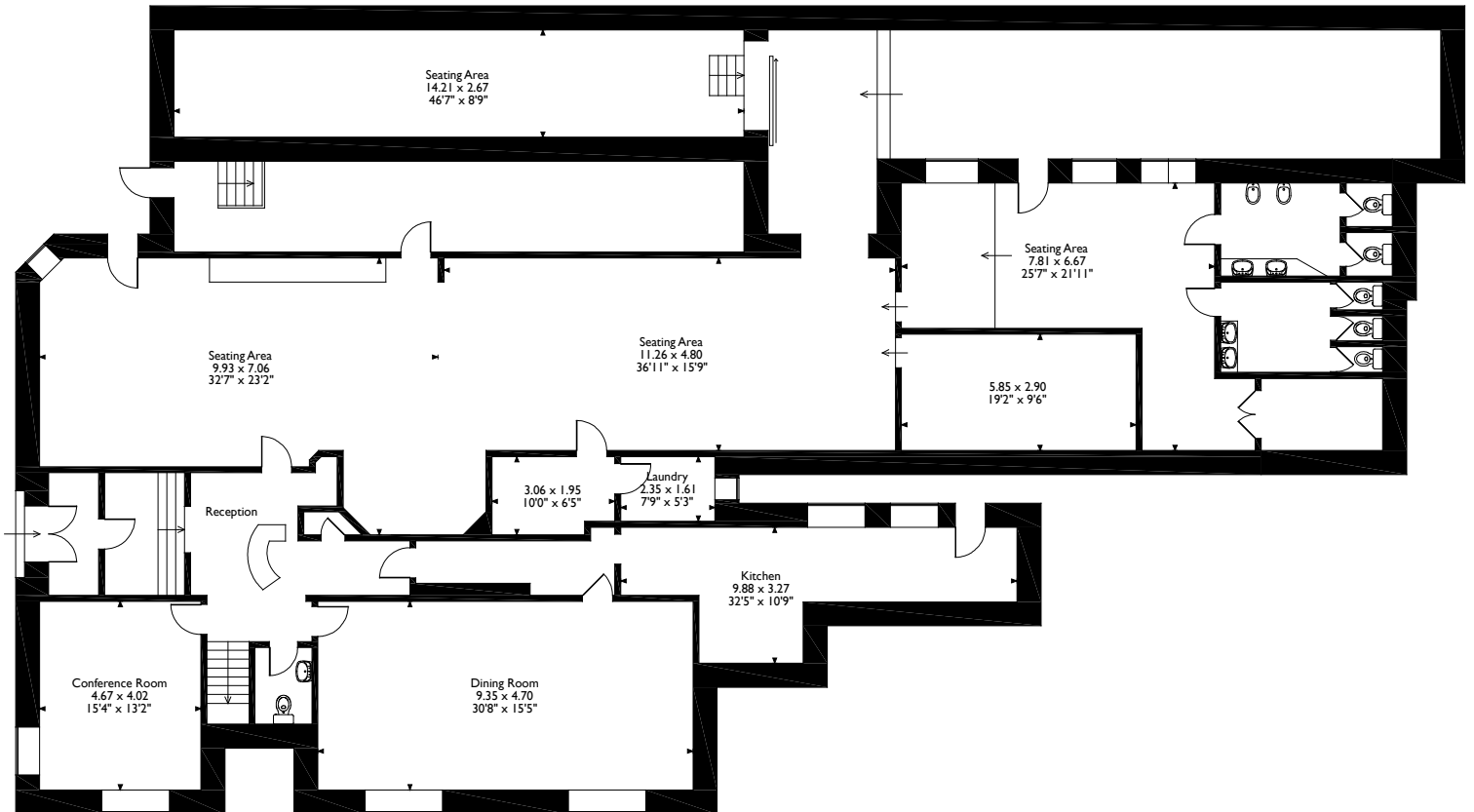
Ground Floor
