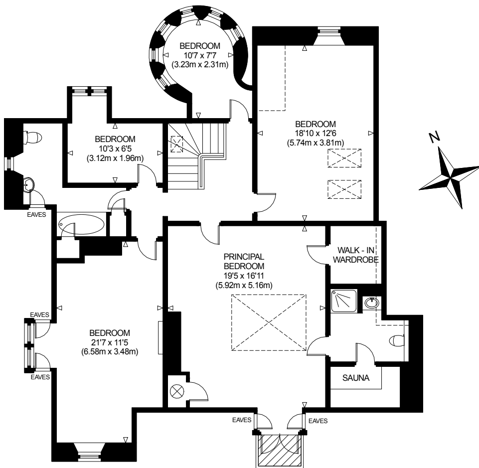
SECOND FLOOR GROSS INTERNAL FLOOR AREA 1352 SQ FT / 125.6 SQ M
