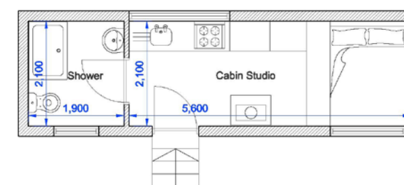
Floor Plan (scale 1:50)
