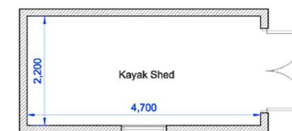
Floor Plan (scale 1:50)
